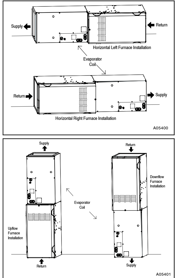
Figure 1 - Typical Coil Installation on Furnace
