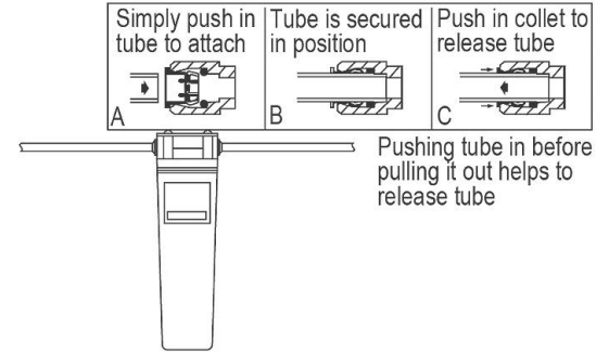
WaterSentry ® Plus Filter System
